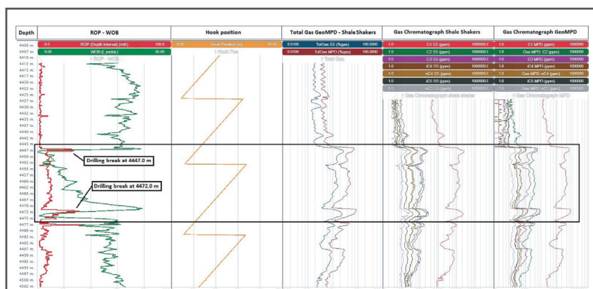
Fig. 4: in the sand interval from xx45.0 m to xx77.0 m a higher gas reading is observed on the GeoMPD.
