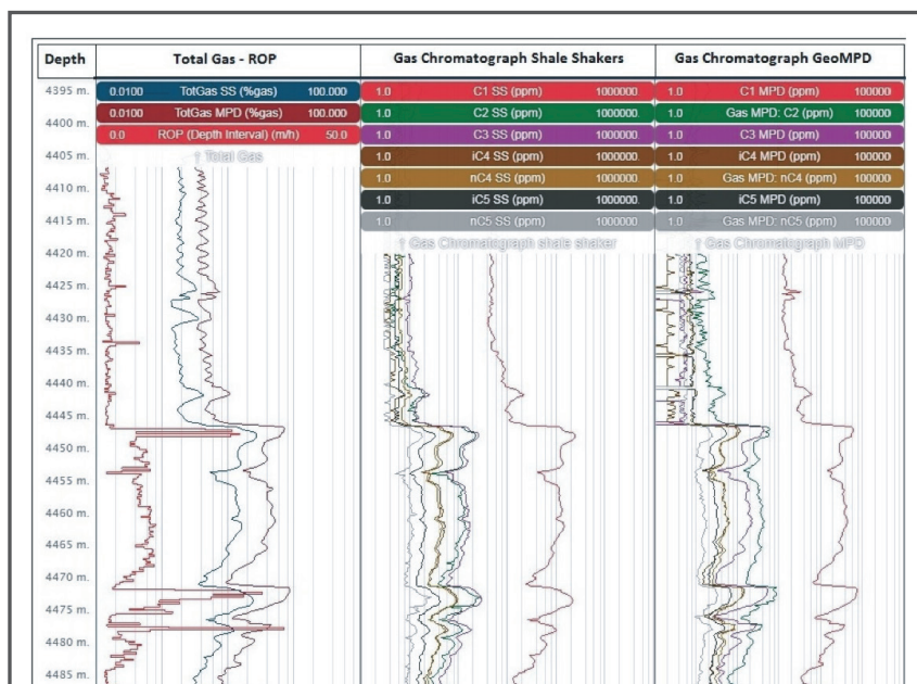
Fig. 5: in the same sand interval, two drilling breaks were observed - the resulting gas from each showed a prompt response on the GeoMPD compared to the readings taken at the shale shakers. This is due to the partial loss of gases at MGS, and the extra air dilution at the shale shakers.
