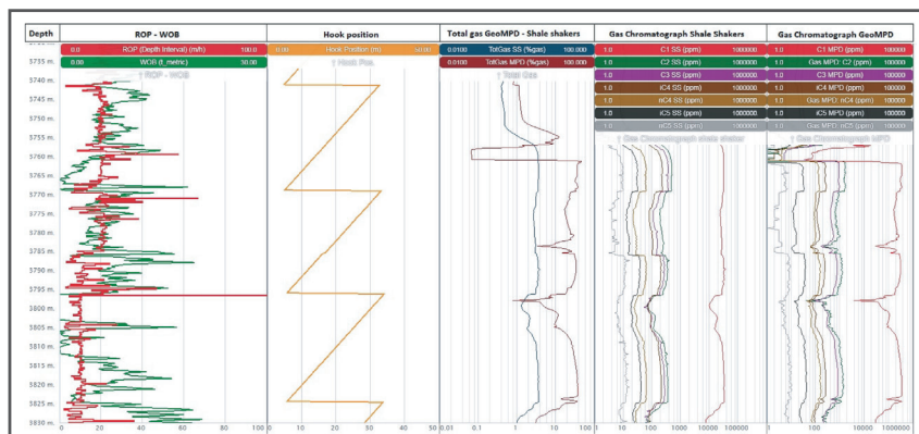
Fig.3: GeoMPD recorded higher gas concentrations as compared to the gas readings of the drilling fluid sampled at the shale shakers; in addition, the relative gas component breakdown is better preserved in the GeoMPD sample compared to shaker sample which is affected by selective gas phase evaporation.
