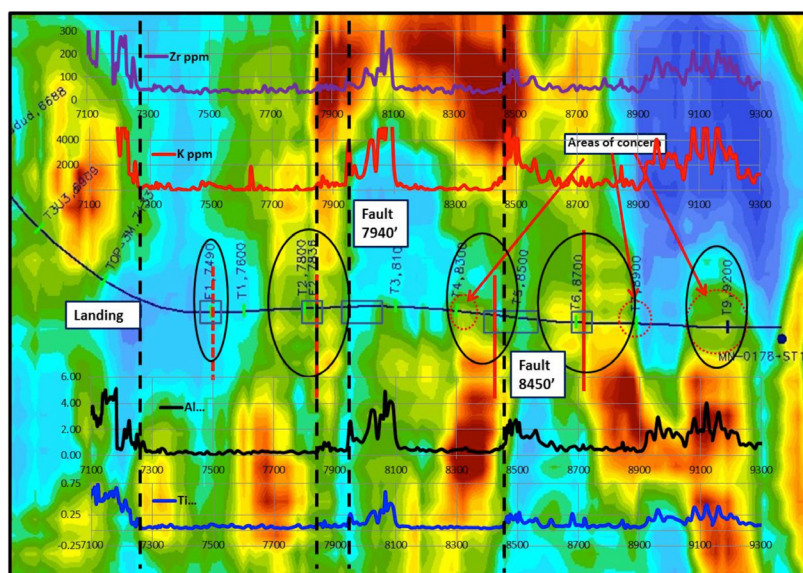
Fig.1 XRF Vs Seismic Data
