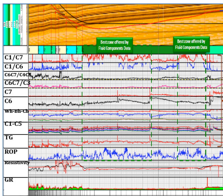
Fig.1 Curtain section combining structural framework with predicted formations alongside actual LWD & GWD responses observed during geosteering a horizontal well
