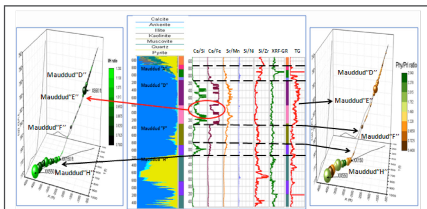
Fig.1 Elemental and mineral Integration with detailed fluid C9-27 hydrocarbon characterization
