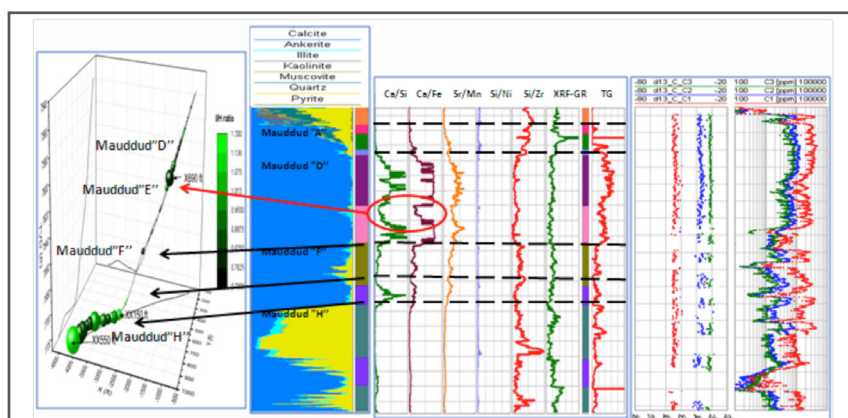
Fig.2, Elemental and mineral integration with detailed fluid C9-27 characterizations isotope analysis C1-C3
